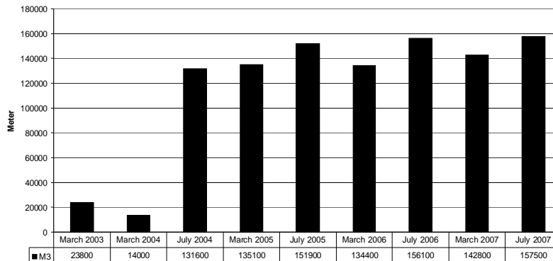
Figure 13. Average beach volume development 70 meter
