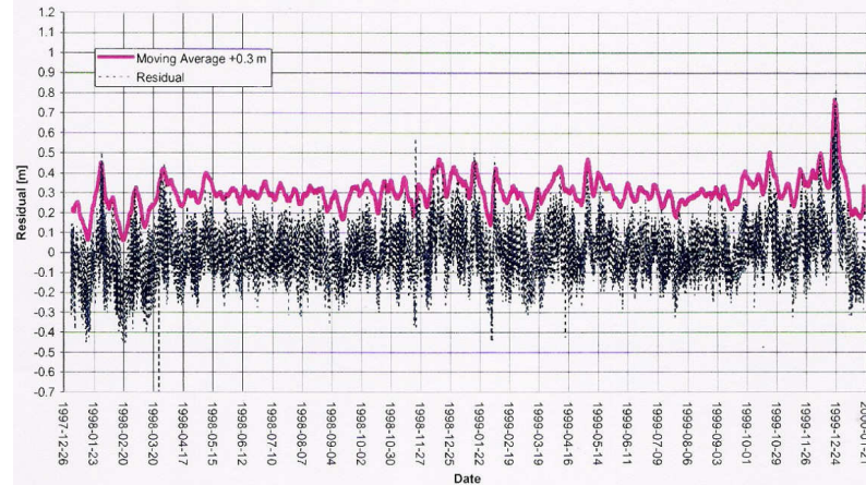
Figure 4. Difference between measured and predicted tide (residual). (Kuantan Port)
