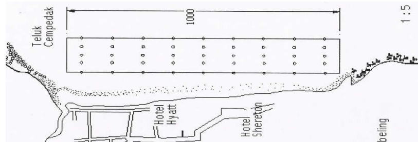
Figure 1a. SIC vertical drain pipe matrix on the beach, 9 columns and 5 rows
